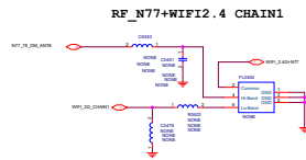
RF_N77+WIFI2.4 CHAIN1
